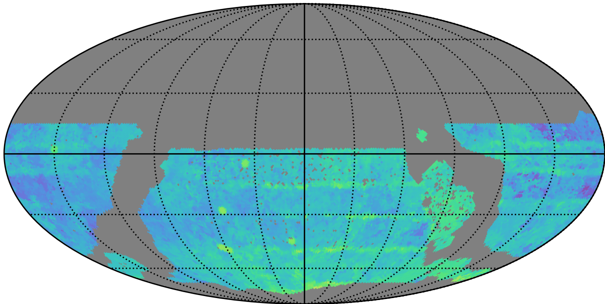
too_5_4v3.4_10yrs WFD r band: Median Season Length
