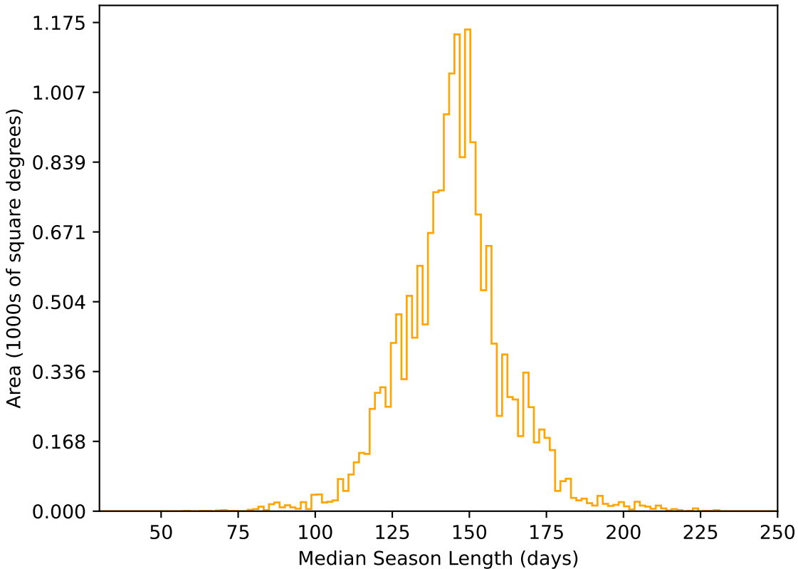
too_5_4v3.4_10yrs WFD r band: Median Season Length
