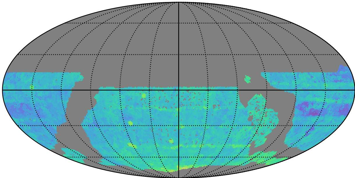
too_5_4v3.4_10yrs WFD i band: Median Season Length
