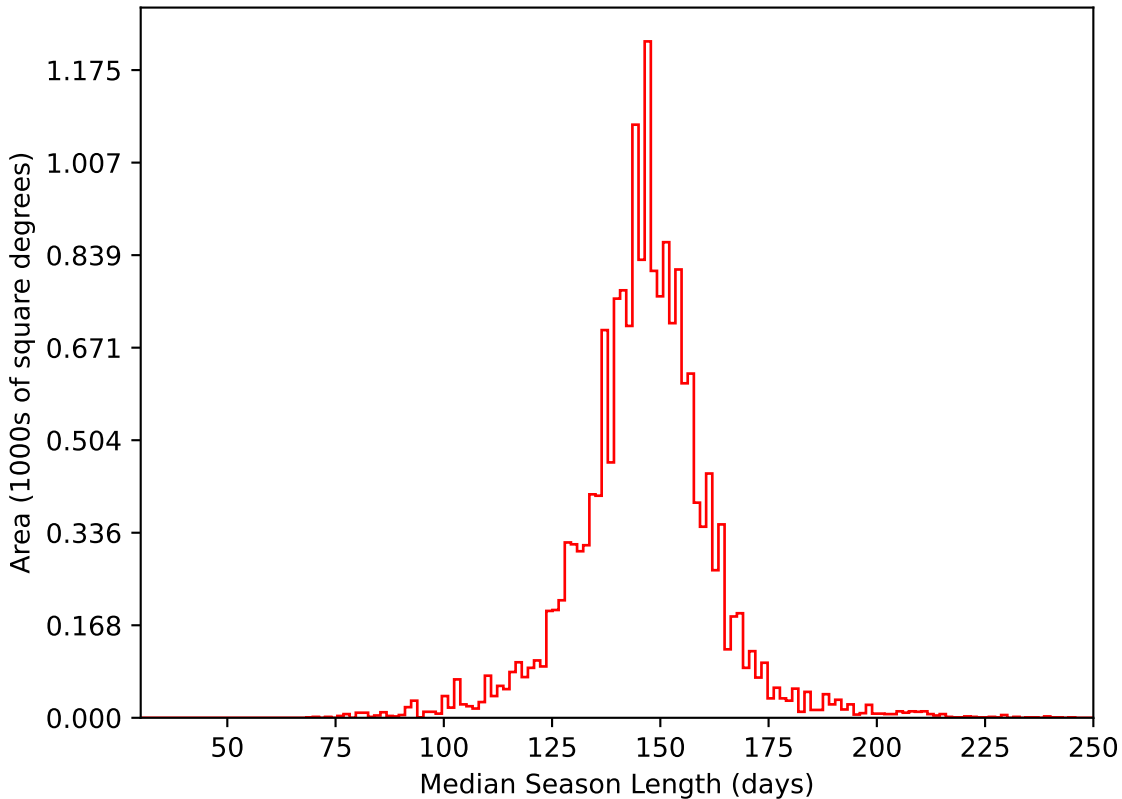
too_5_4v3.4_10yrs WFD i band: Median Season Length
