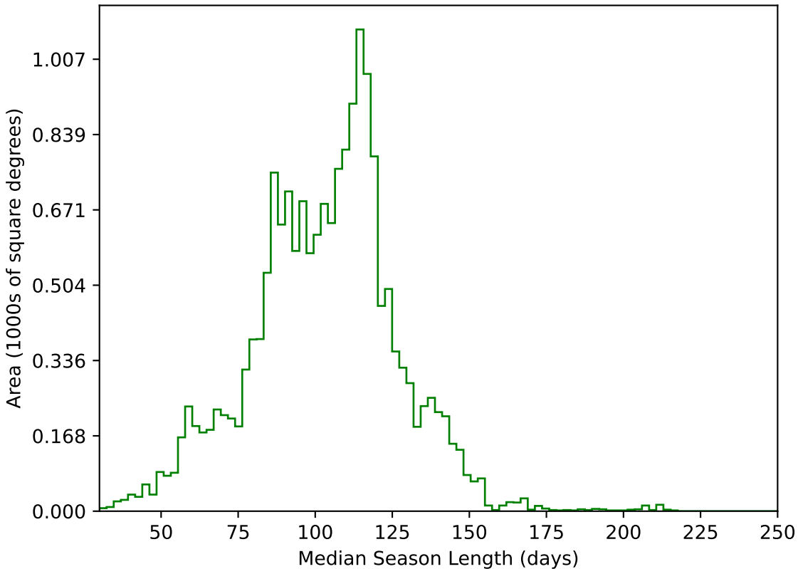
too_5_4v3.4_10yrs WFD g band: Median Season Length
