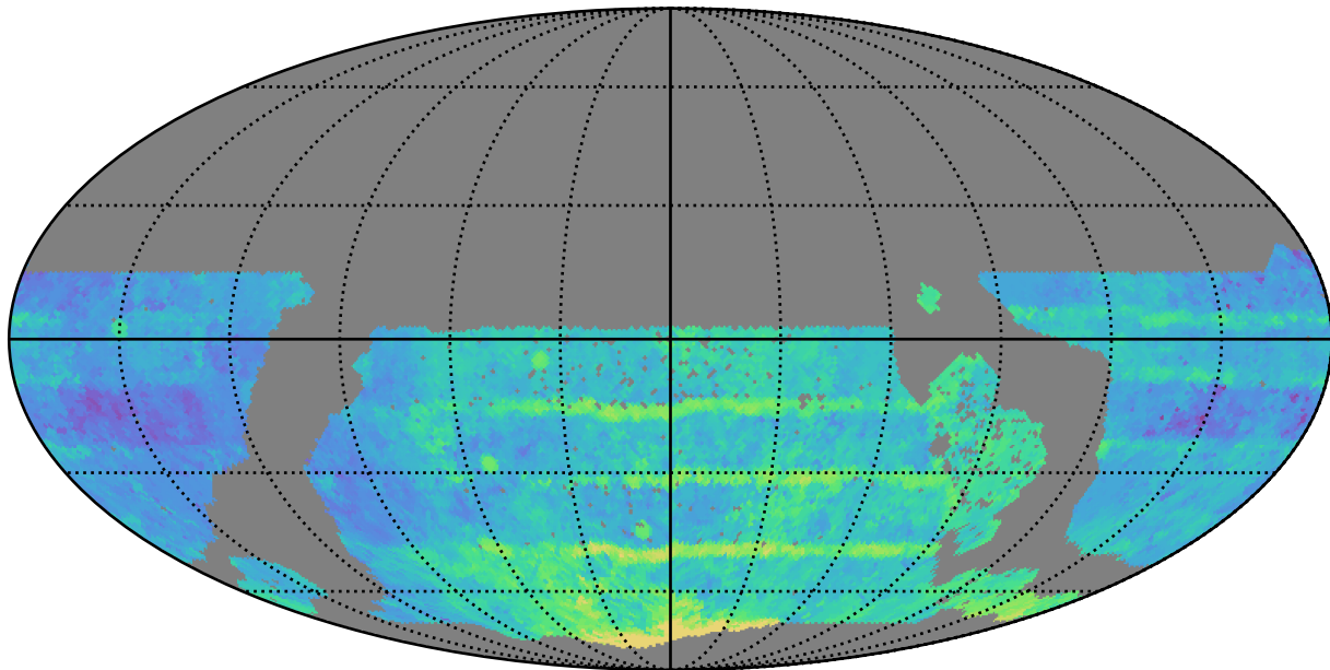
too_5_4v3.4_10yrs WFD all bands: Median Season Length
