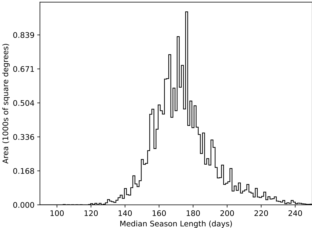
too_5_4v3.4_10yrs WFD all bands: Median Season Length
