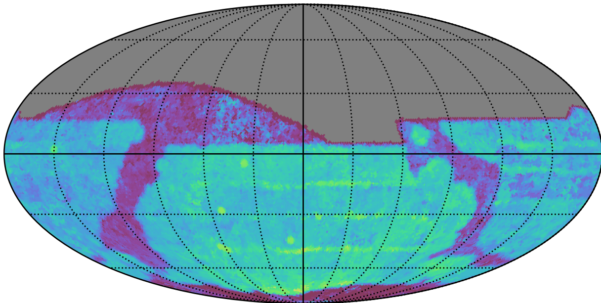
too_5_4v3.4_10yrs All sky z band: Median Season Length
