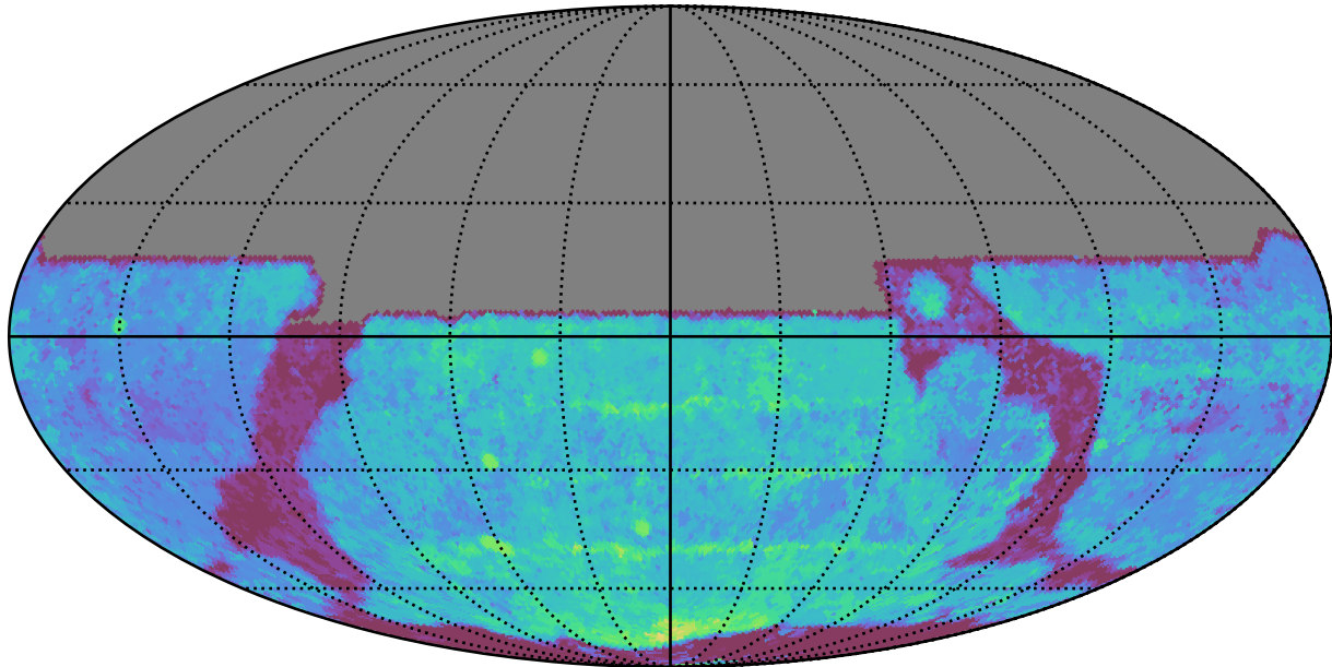
too_5_4v3.4_10yrs All sky y band: Median Season Length
