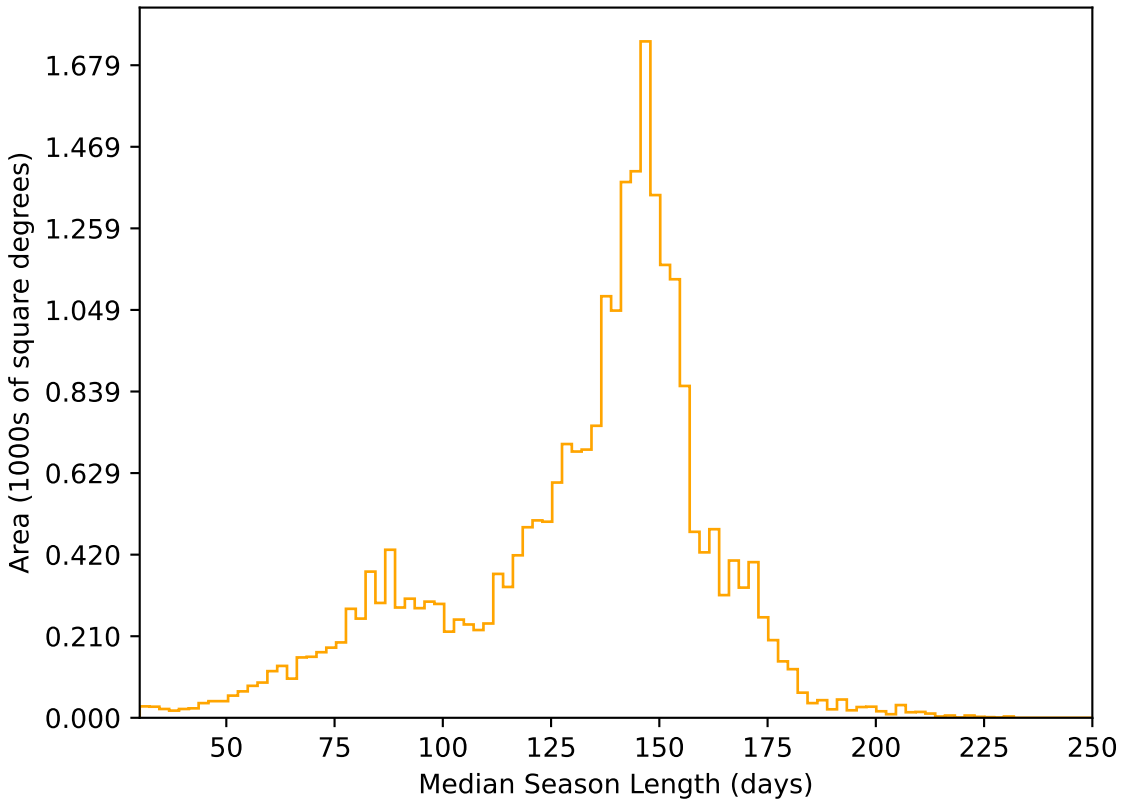
too_5_4v3.4_10yrs All sky r band: Median Season Length
