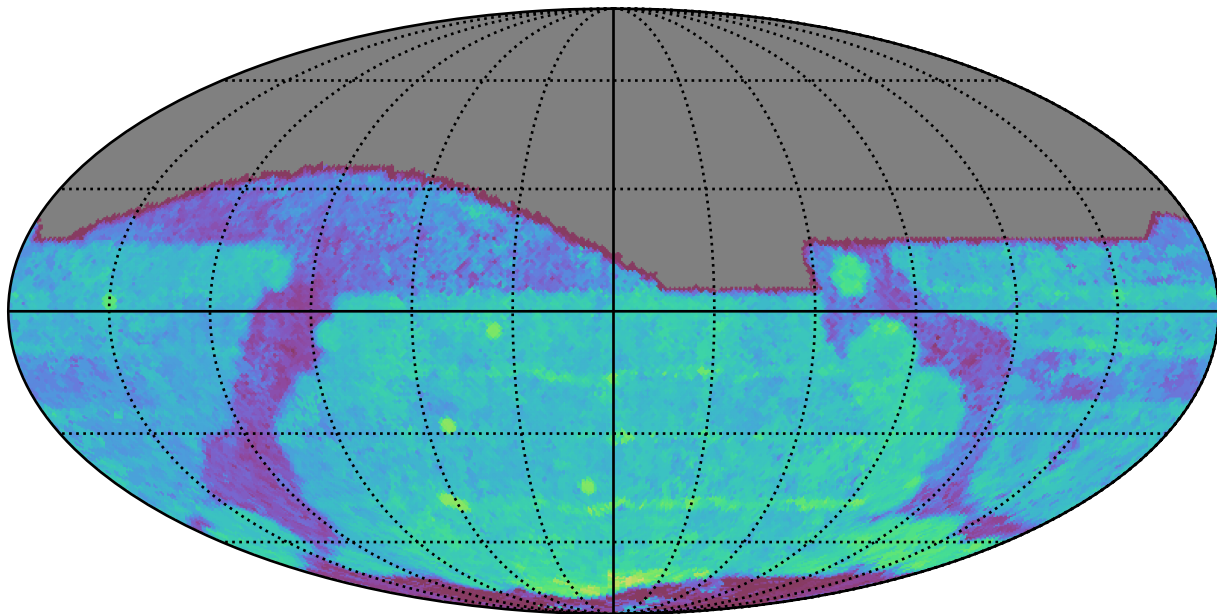
too_5_4v3.4_10yrs All sky i band: Median Season Length
