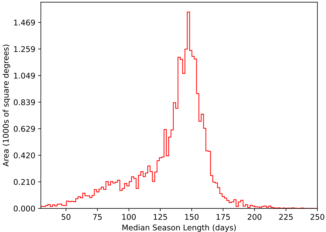
too_5_4v3.4_10yrs All sky i band: Median Season Length
