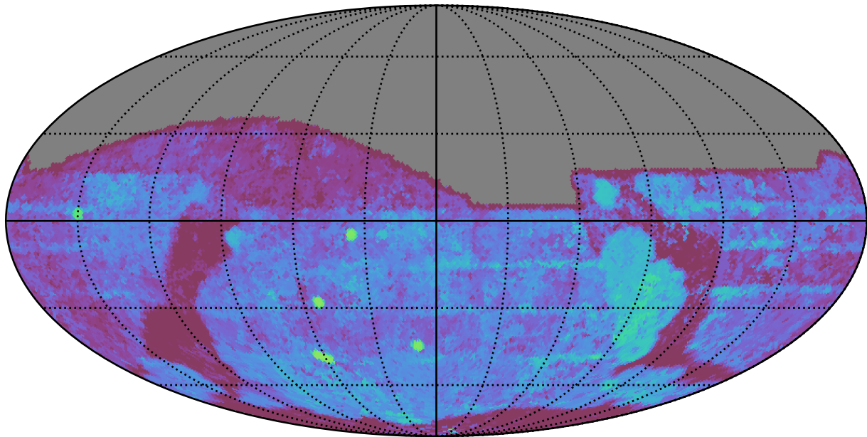
too_5_4v3.4_10yrs All sky g band: Median Season Length
