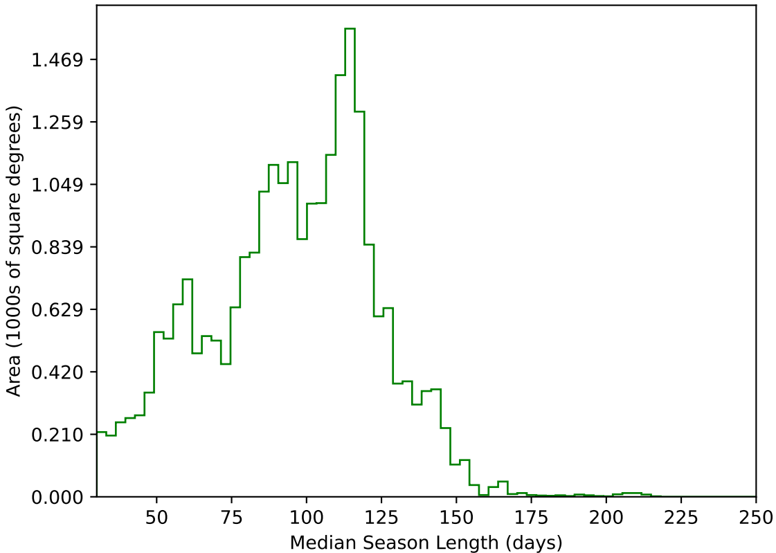
too_5_4v3.4_10yrs All sky g band: Median Season Length
