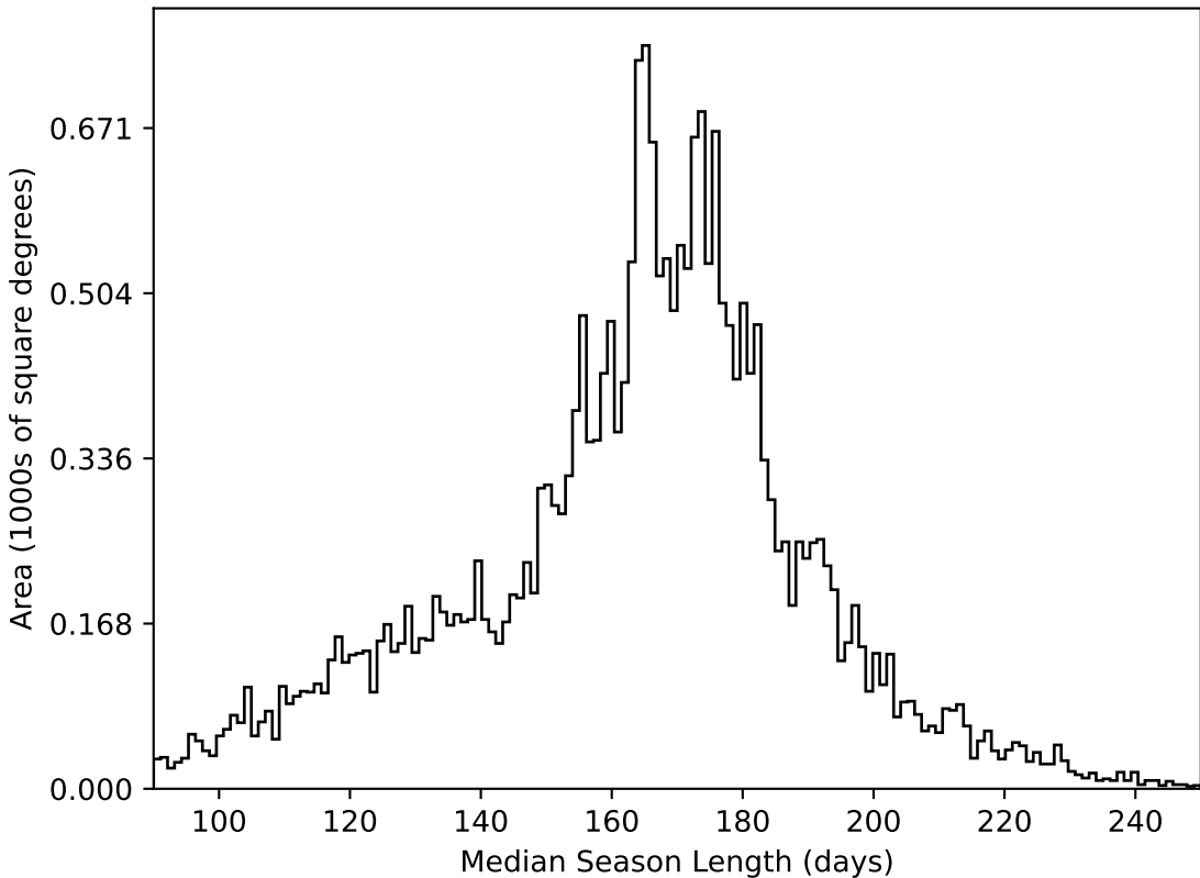
too_5_4v3.4_10yrs All sky all bands: Median Season Length
