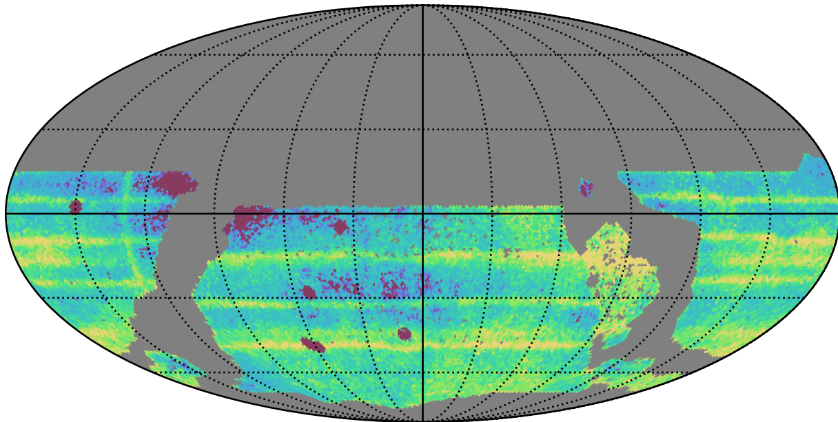
too_5_4v3.4_10yrs WFD: Median Intra-Night Gap
