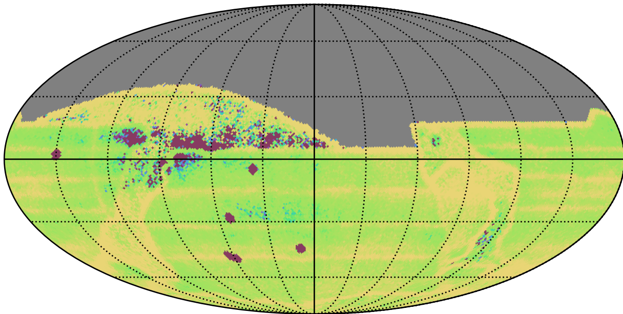
too_5_4v3.4_10yrs All sky: Median Intra-Night Gap
