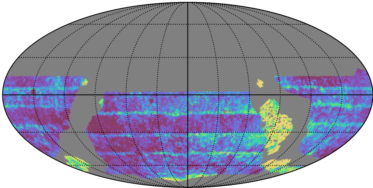
too_5_4v3.4_10yrs WFD z band: Median Inter-Night Gap
