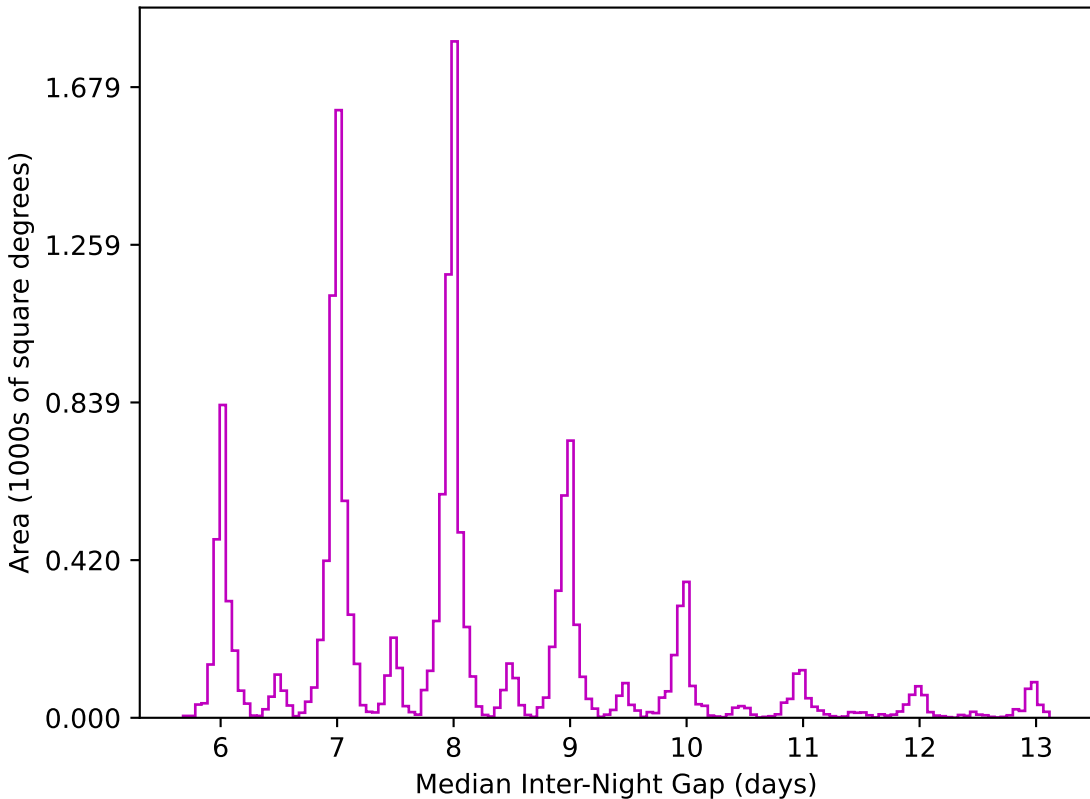
too_5_4v3.4_10yrs WFD z band: Median Inter-Night Gap
