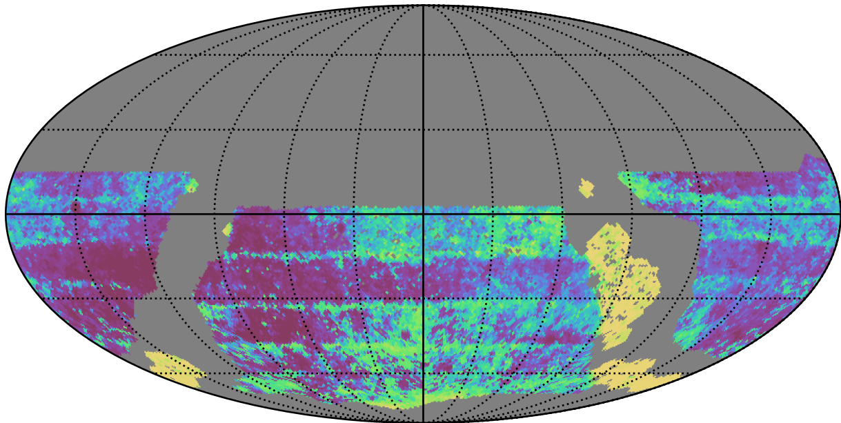
too_5_4v3.4_10yrs WFD y band: Median Inter-Night Gap
