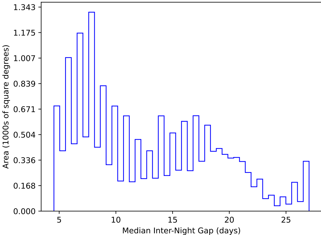
too_5_4v3.4_10yrs WFD y band: Median Inter-Night Gap
