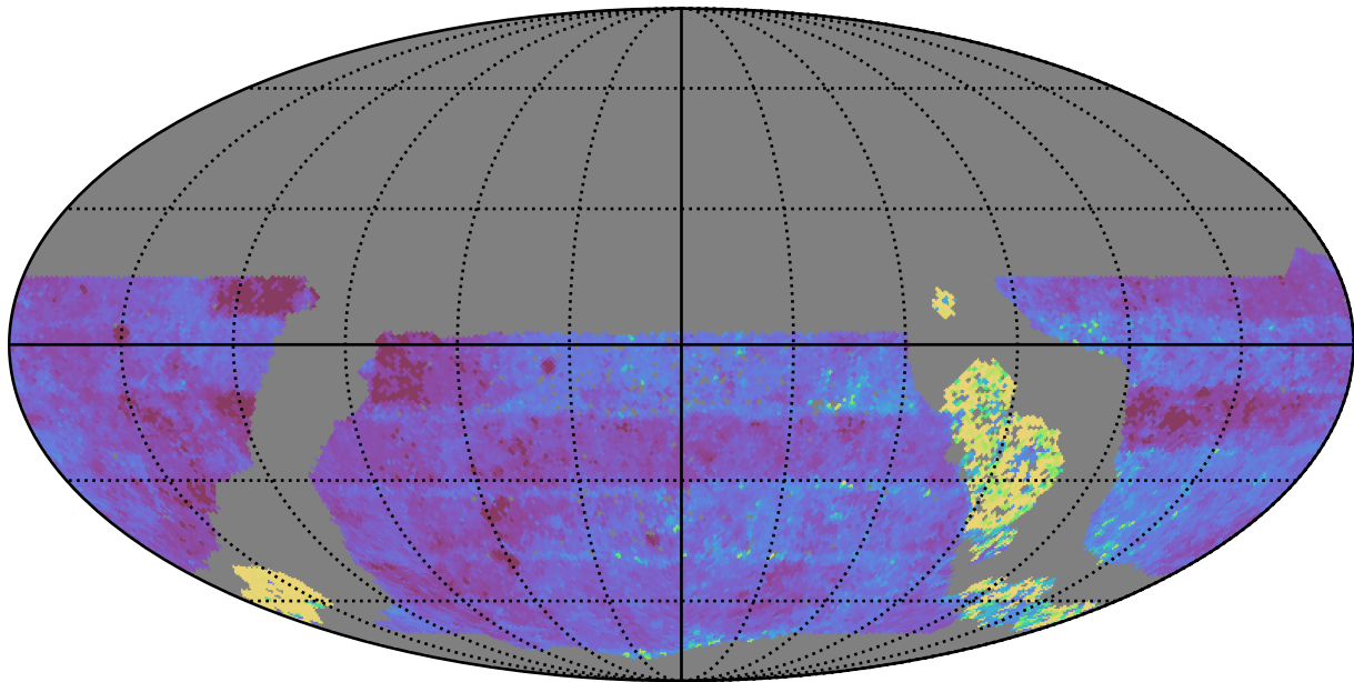
too_5_4v3.4_10yrs WFD u band: Median Inter-Night Gap
