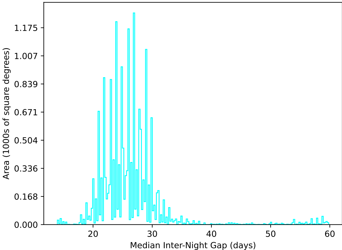
too_5_4v3.4_10yrs WFD u band: Median Inter-Night Gap
