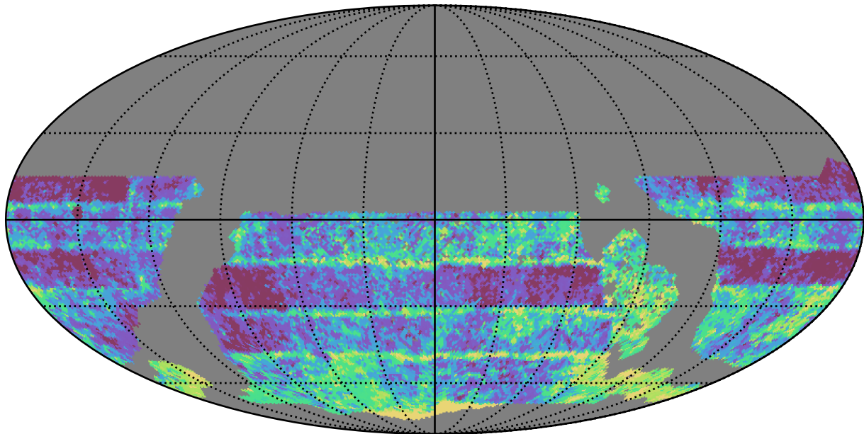
too_5_4v3.4_10yrs WFD r band: Median Inter-Night Gap
