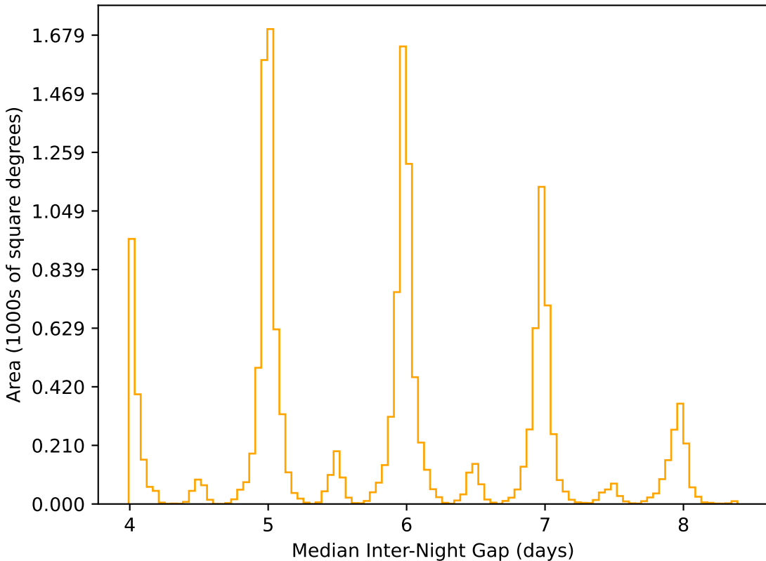
too_5_4v3.4_10yrs WFD r band: Median Inter-Night Gap
