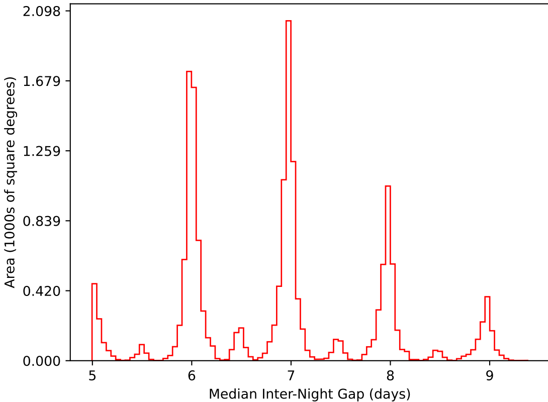
too_5_4v3.4_10yrs WFD i band: Median Inter-Night Gap
