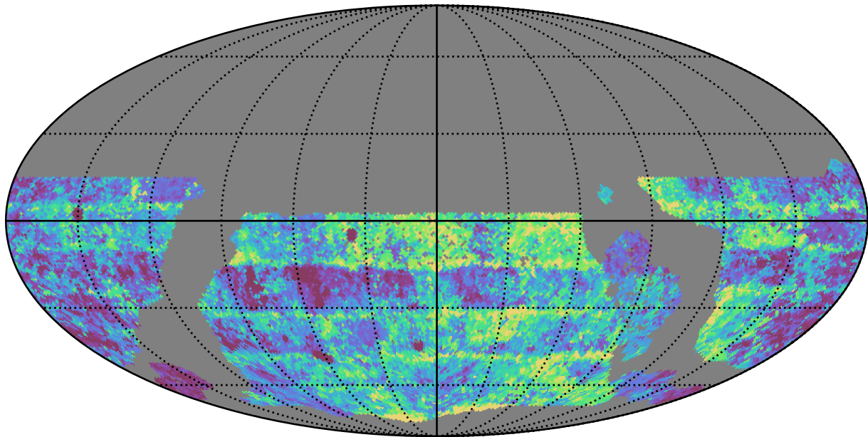
too_5_4v3.4_10yrs WFD g band: Median Inter-Night Gap
