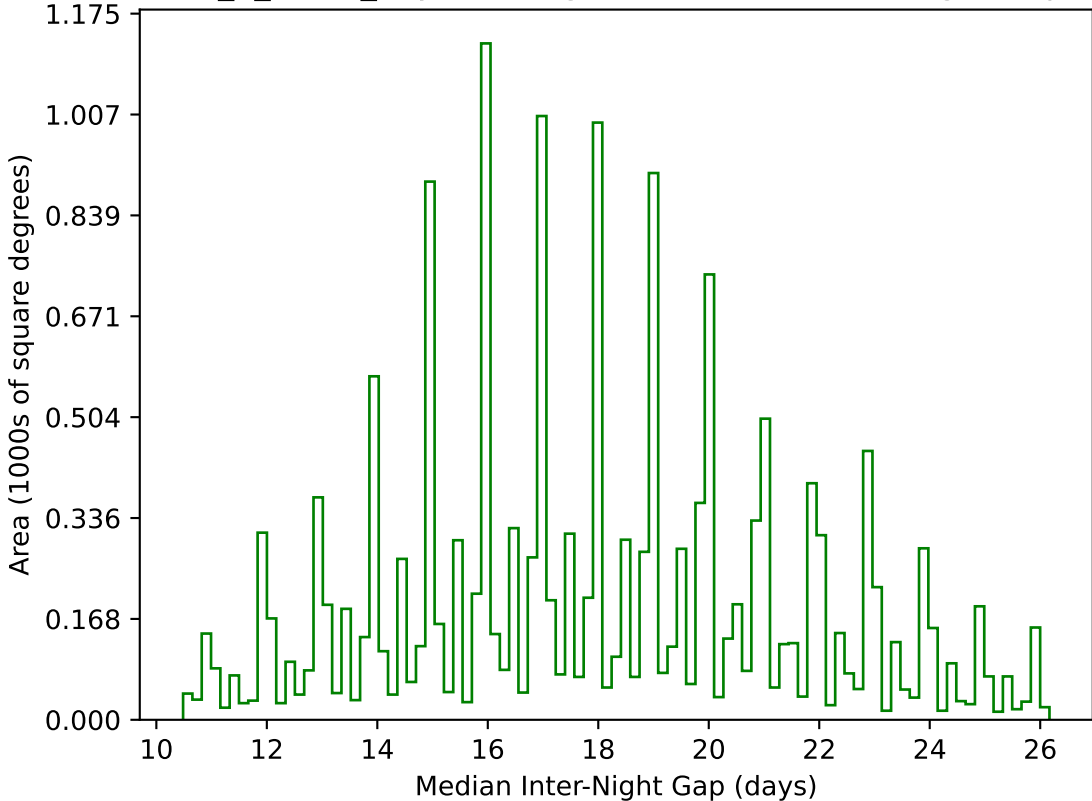
too_5_4v3.4_10yrs WFD g band: Median Inter-Night Gap
