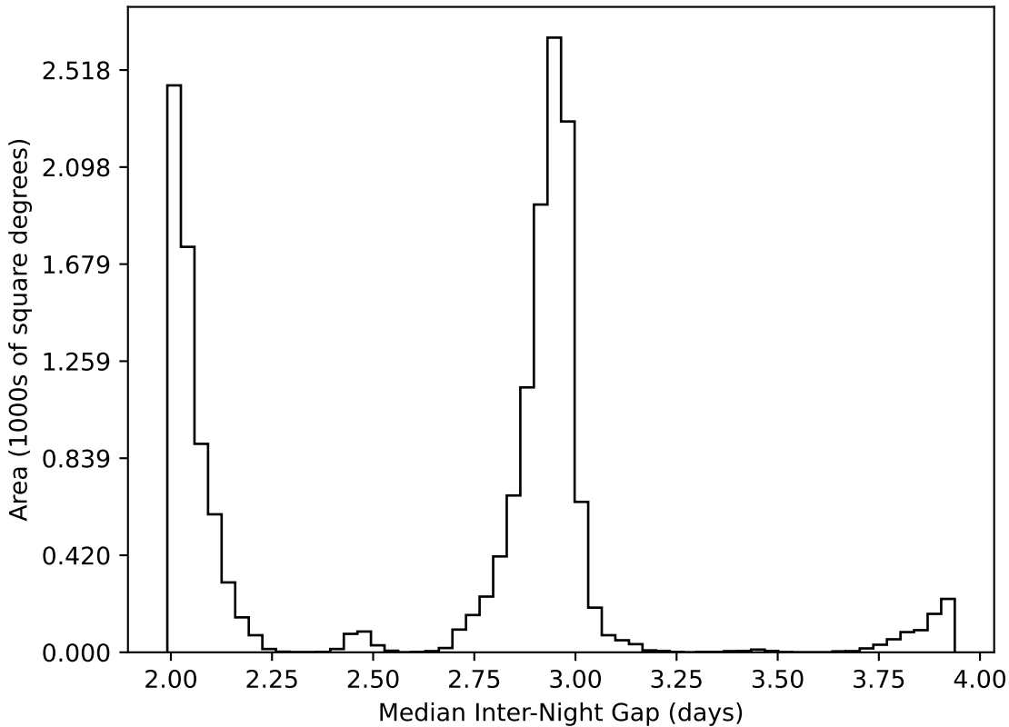
too_5_4v3.4_10yrs WFD all bands: Median Inter-Night Gap
