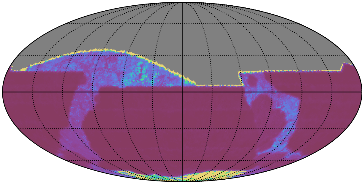
too_5_4v3.4_10yrs All sky z band: Median Inter-Night Gap
