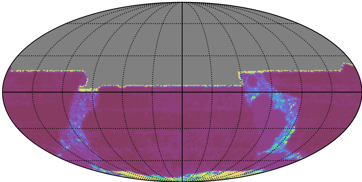
too_5_4v3.4_10yrs All sky y band: Median Inter-Night Gap
