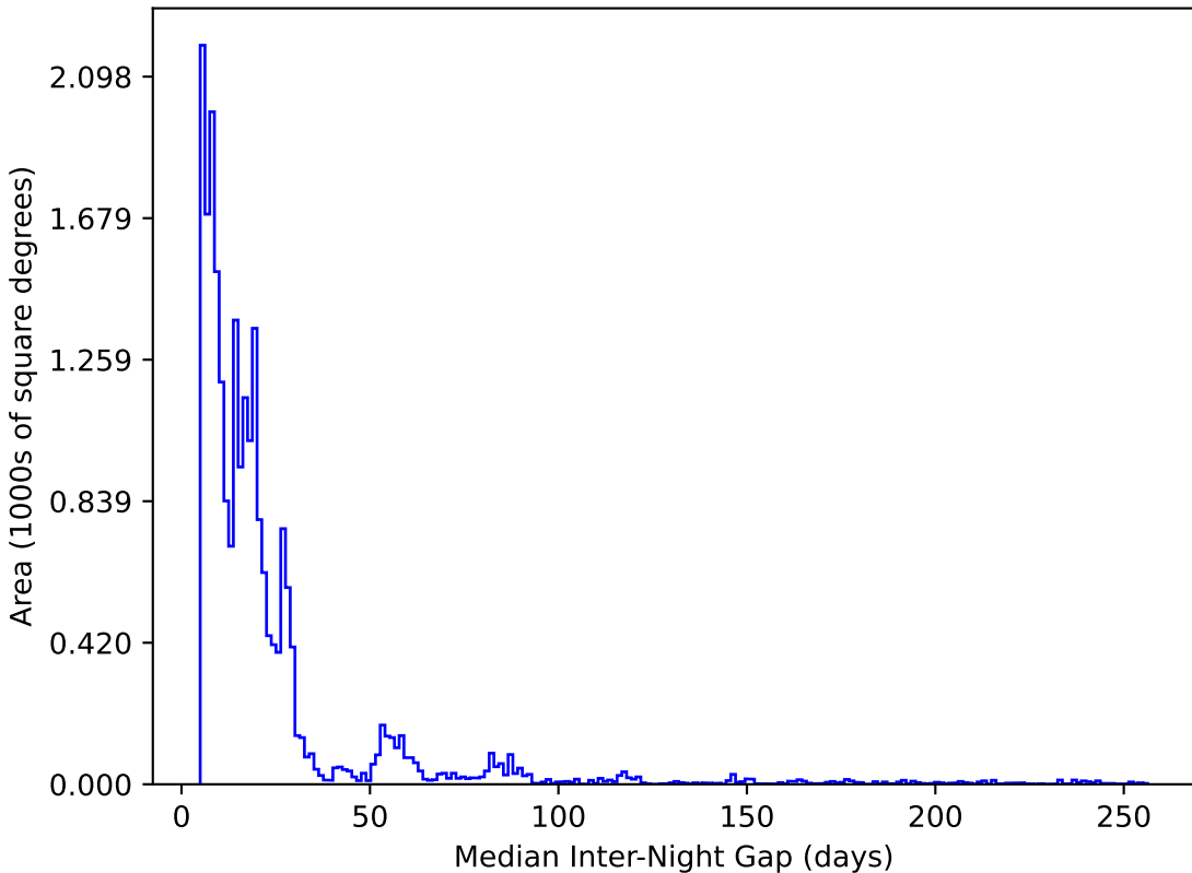
too_5_4v3.4_10yrs All sky y band: Median Inter-Night Gap
