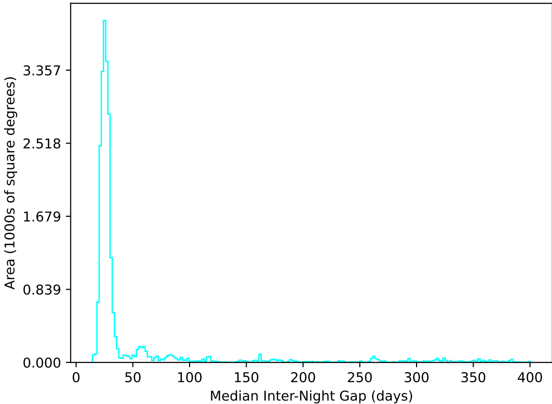
too_5_4v3.4_10yrs All sky u band: Median Inter-Night Gap
