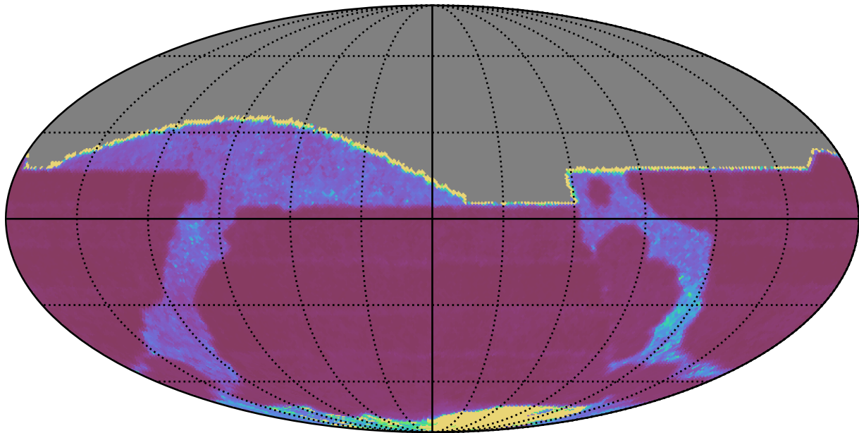
too_5_4v3.4_10yrs All sky r band: Median Inter-Night Gap
