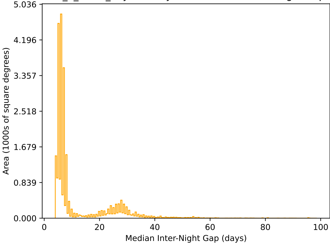
too_5_4v3.4_10yrs All sky r band: Median Inter-Night Gap
