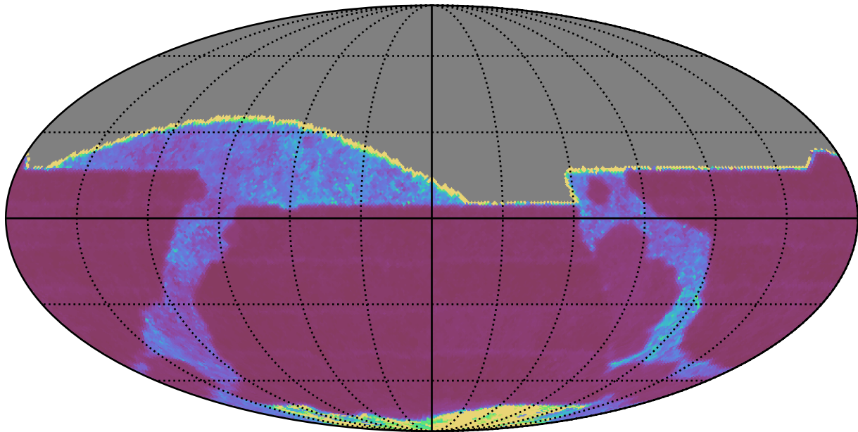
too_5_4v3.4_10yrs All sky i band: Median Inter-Night Gap
