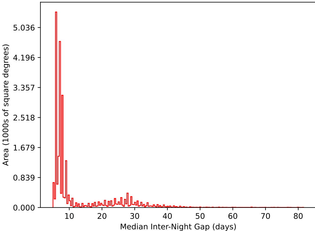
too_5_4v3.4_10yrs All sky i band: Median Inter-Night Gap
