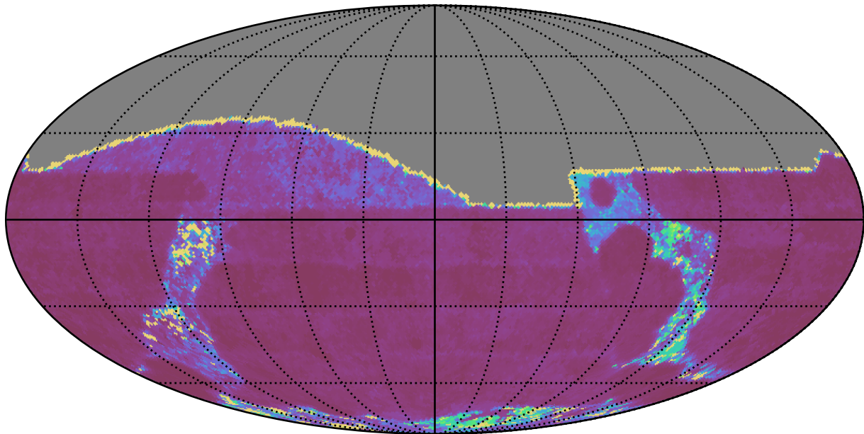
too_5_4v3.4_10yrs All sky g band: Median Inter-Night Gap
