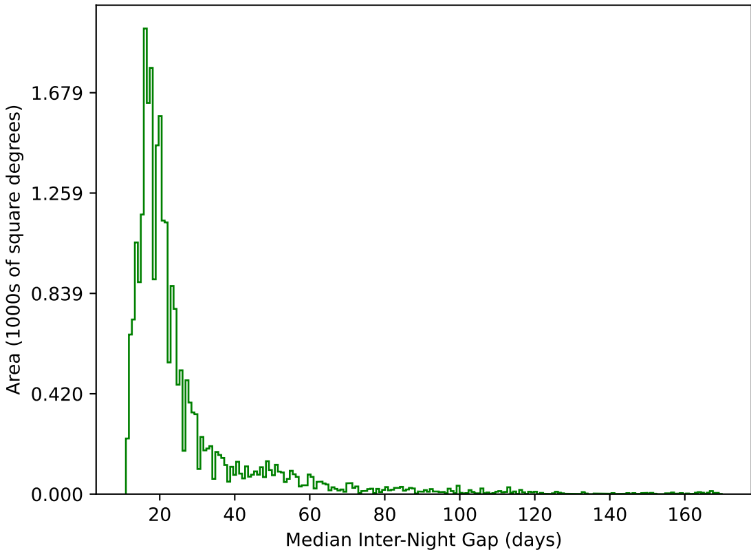
too_5_4v3.4_10yrs All sky g band: Median Inter-Night Gap
