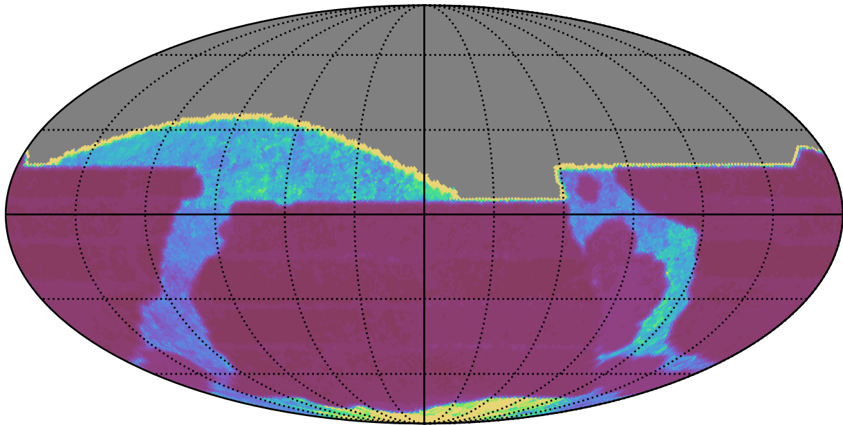
too_5_4v3.4_10yrs All sky all bands: Median Inter-Night Gap
