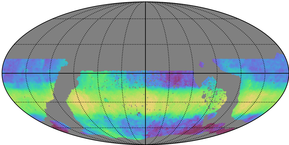
too_5_4v3.4_10yrs WFD z band: Median HA
