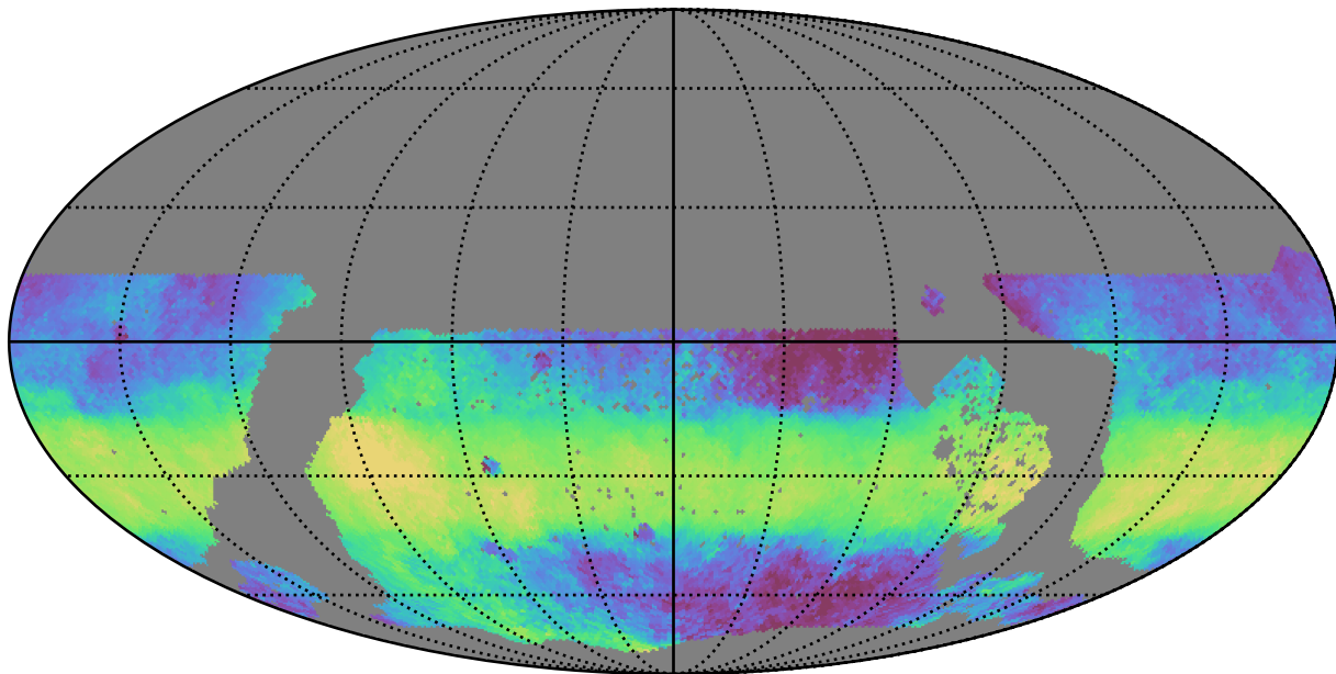
too_5_4v3.4_10yrs WFD y band: Median HA
