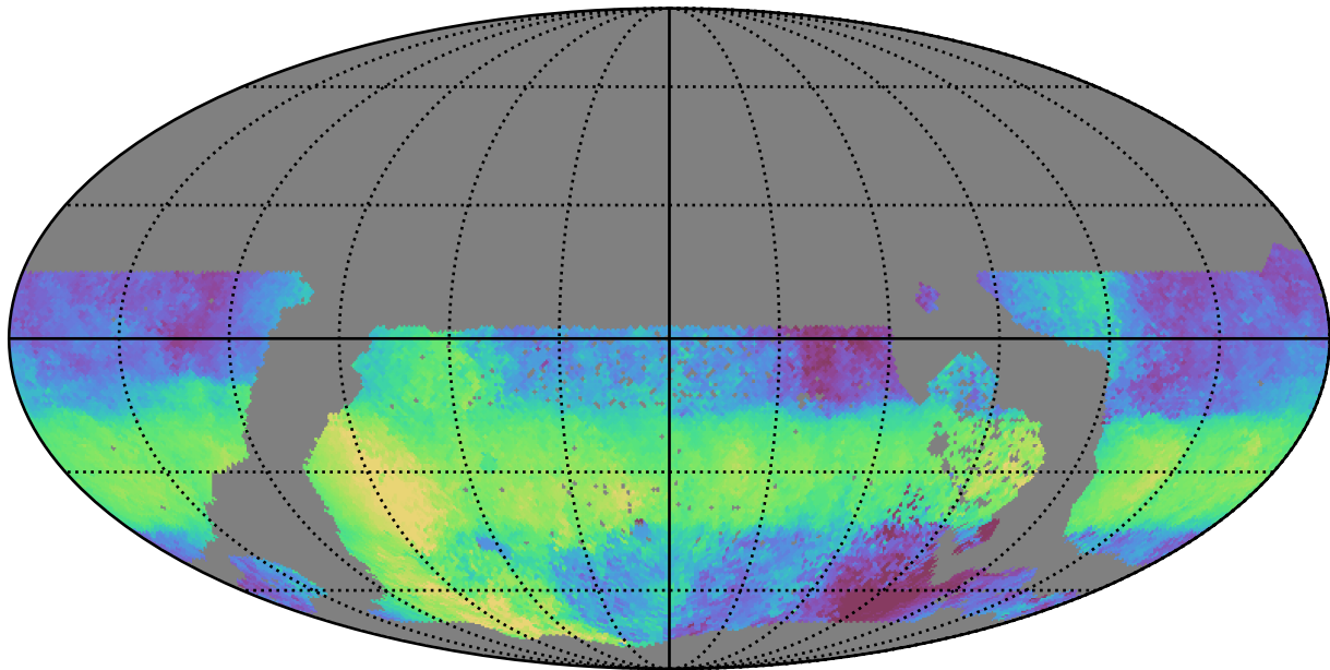
too_5_4v3.4_10yrs WFD u band: Median HA
