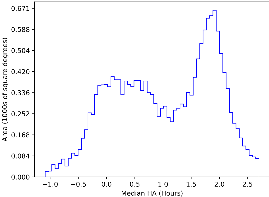
too_5_4v3.4_10yrs WFD u band: Median HA
