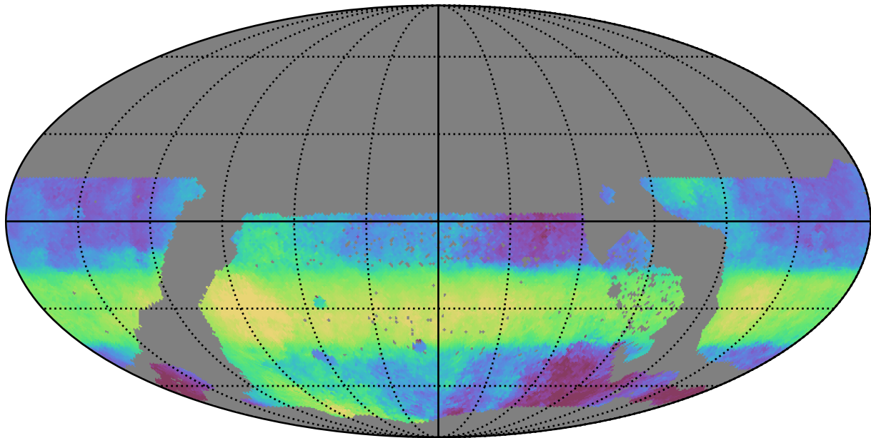
too_5_4v3.4_10yrs WFD r band: Median HA
