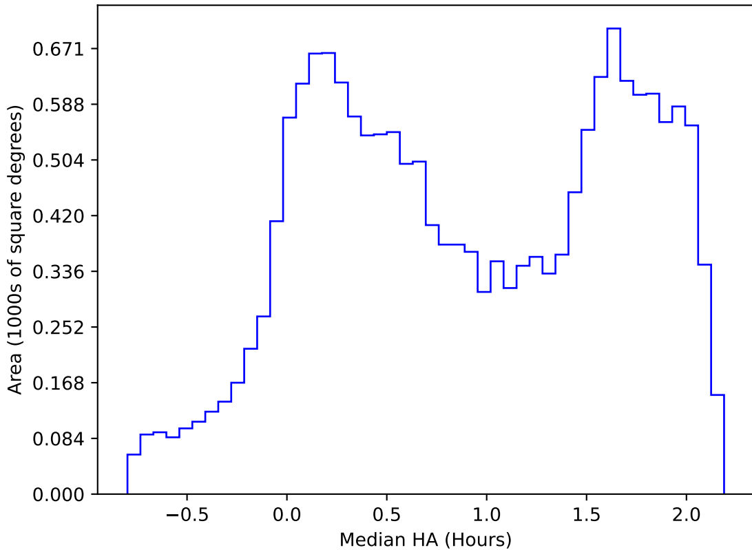
too_5_4v3.4_10yrs WFD r band: Median HA
