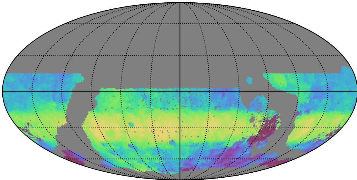
too_5_4v3.4_10yrs WFD g band: Median HA
