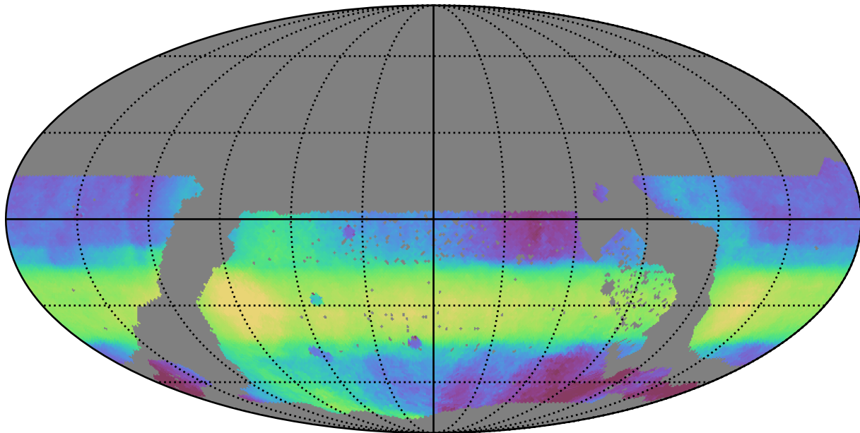
too_5_4v3.4_10yrs WFD all bands: Median HA
