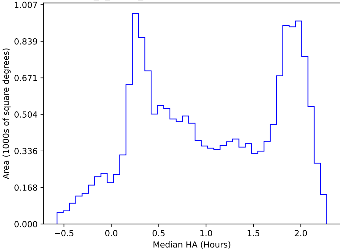
too_5_4v3.4_10yrs WFD all bands: Median HA
