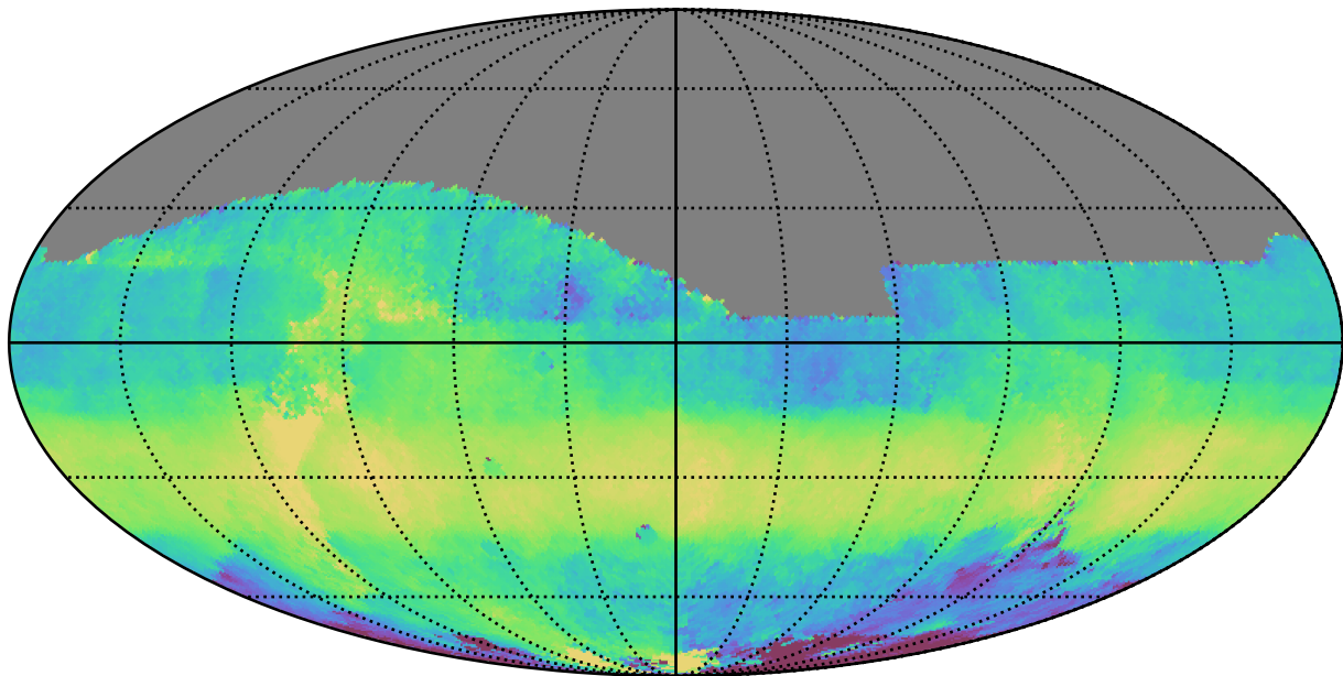
too_5_4v3.4_10yrs All sky z band: Median HA
